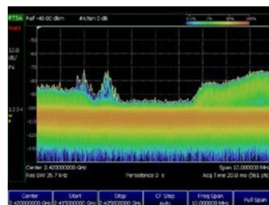
Identify multiple types of signals in the same band (Bluetooth and WiFi)
