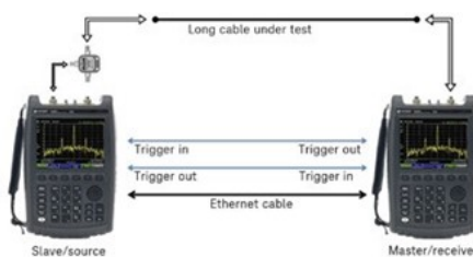
Measure long, lossy cables using ERTA
