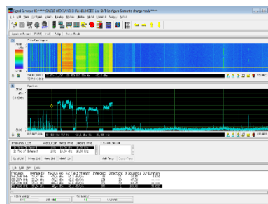
Portable monitoring system covering VLF to 5G millimeter wave bands
