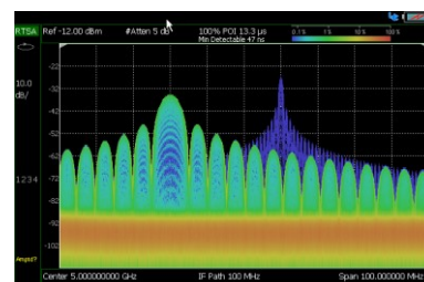
Multi-pulse detection using density display with settable persistence
