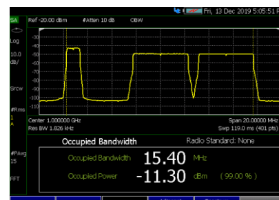
LTE-A occupied bandwidth measurement
