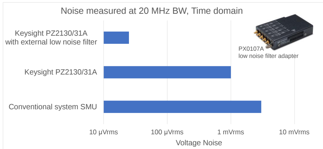
Figure 11. PX0107A dramatically reduce output noise
