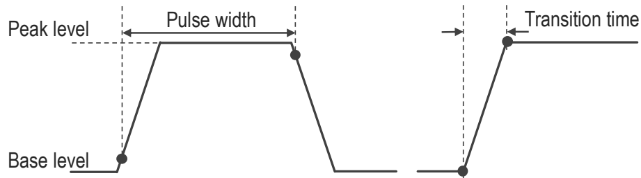
Figure 23. Definition of the pulse parameters and the transition time
