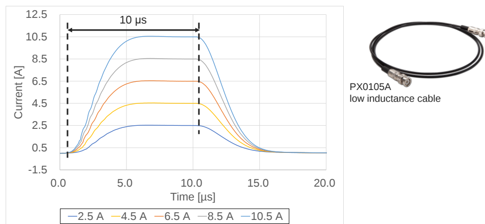
Figure 9. 10 \mu s narrow pulse output with measuring at 15 MSa/s sampling rate
