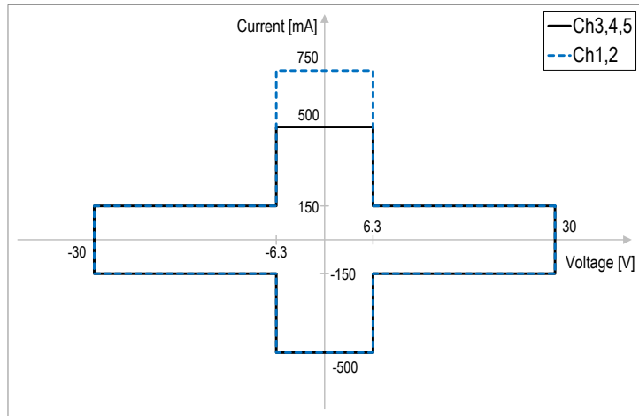
Figure 19. PZ2130/31A voltage and current output capability per channel
