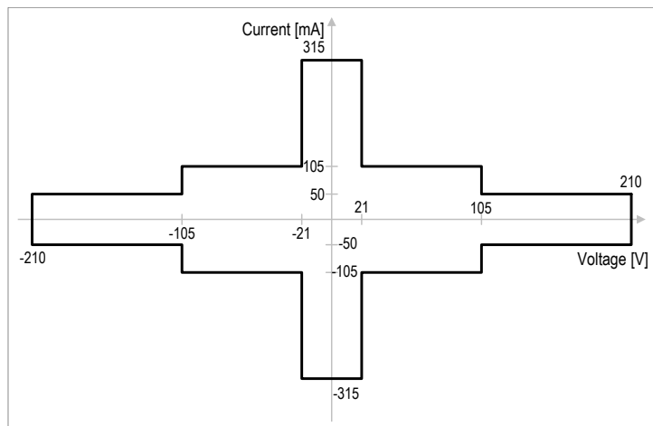
Figure 16. PZ2110A DC voltage and current output capability
