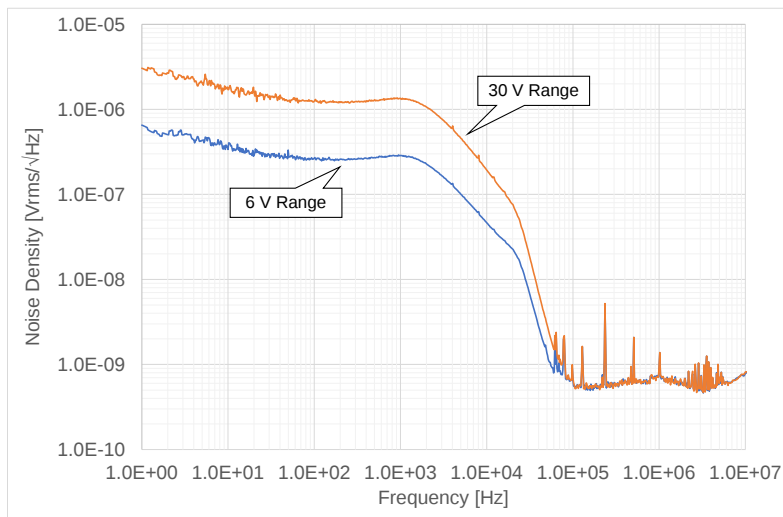
Figure 22. Voltage source noise density of the PZ2130/31A with the PX0107A external low noise filter (Observed data)
