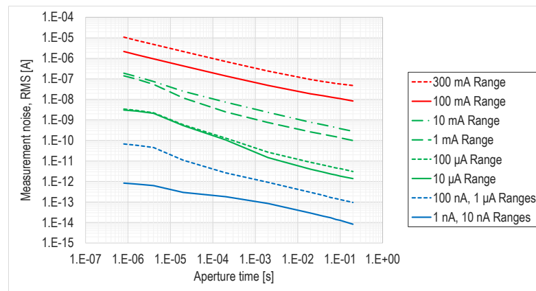
Figure 21. Current measurement noise
