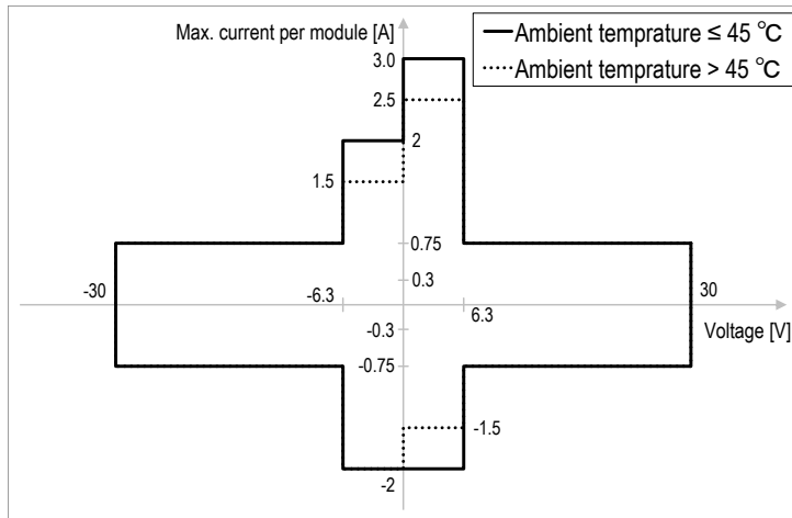
Figure 20. PZ2130/31A voltage and total current output capability per module
