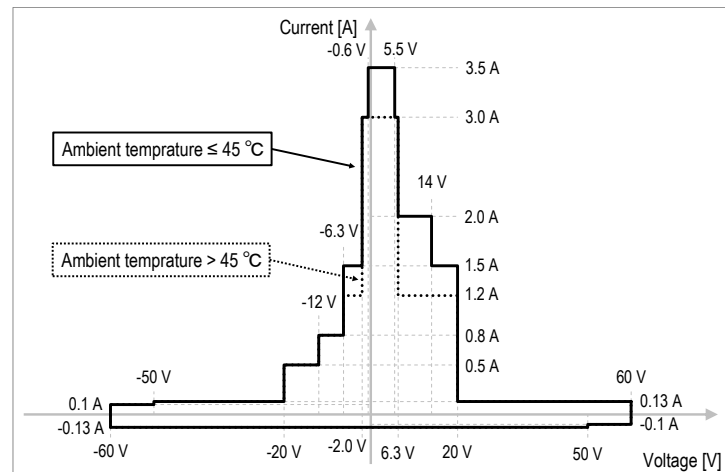
Figure 17. PZ2120/21A DC voltage and current output capability
